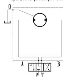
液压原理图 Hydraulic principle diagram
